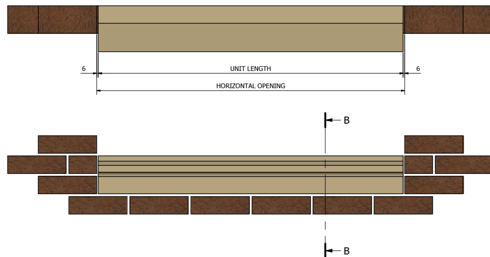
'PWS' TYPE SLIP CILL (170mm x 140mm) ( 1:5 )
