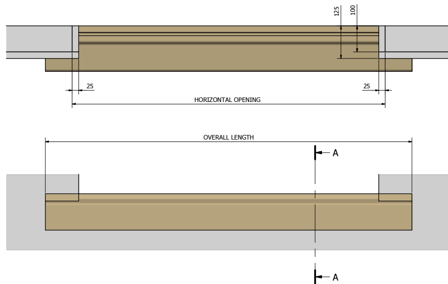
'SR' TYPE STOOLED CILL IN RENDER (175mm x 140mm) ( 1:5 )
