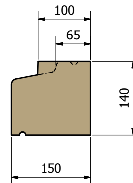
'SC' TYPE WET CAST PROFILE ( 1 : 5 )
