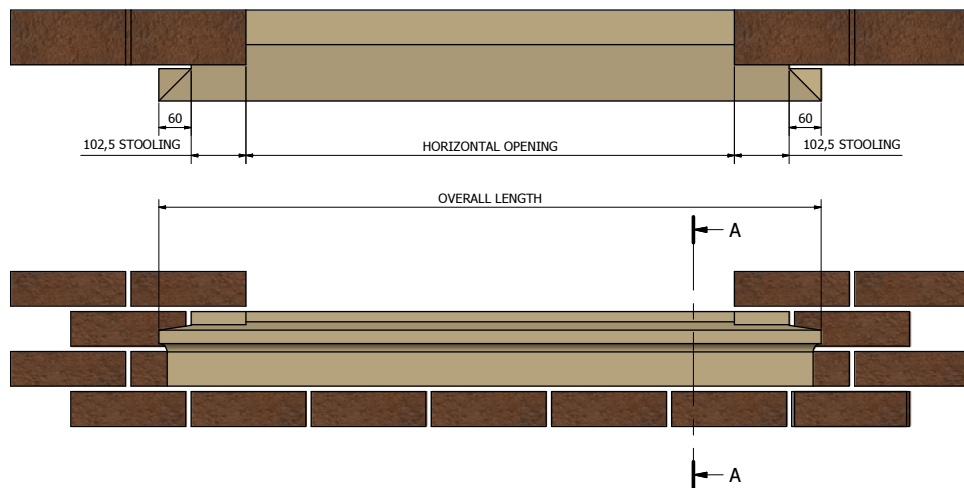
'PW' TYPE STOOLED CILL (170mm x 140mm) ( 1:5 )
