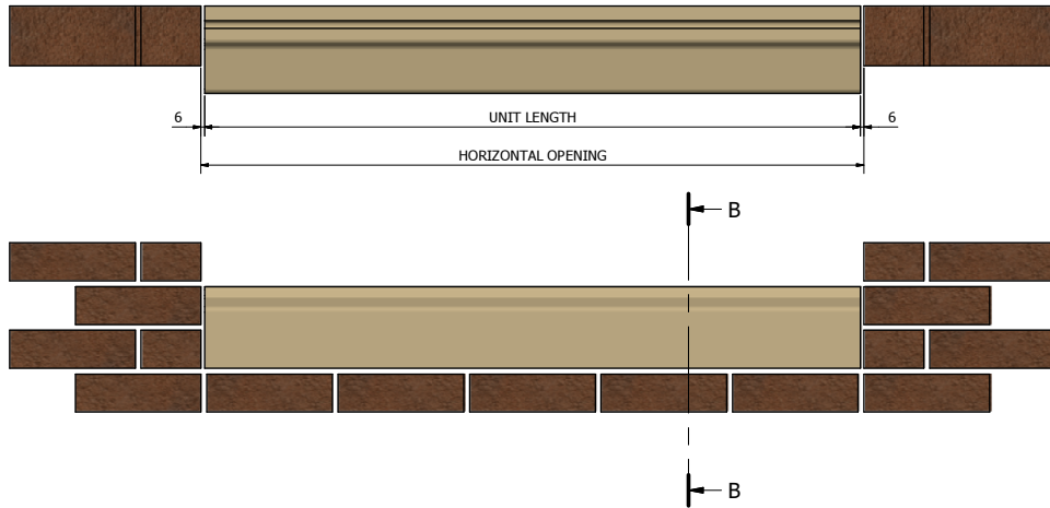
'SCS' TYPE SLIP CILL (150mm x 140mm) ( 1:5 )
