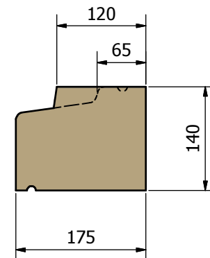
'SR' TYPE WET CAST PROFILE ( 1 : 5 )
