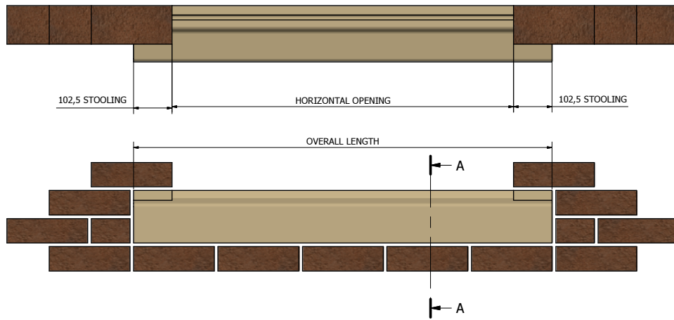
'SC' TYPE STOOLED CILL (150mm x 140mm) ( 1:5 )
