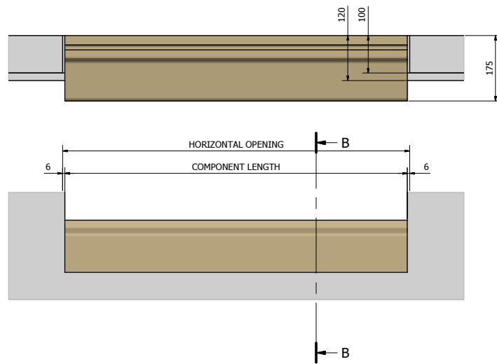
'SRS' TYPE SLIP CILL IN RENDER (175mm x 140mm) ( 1:5 )
