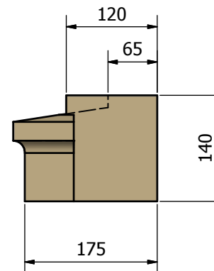
'PWR' TYPE PROFILE ( 1 : 5 )
