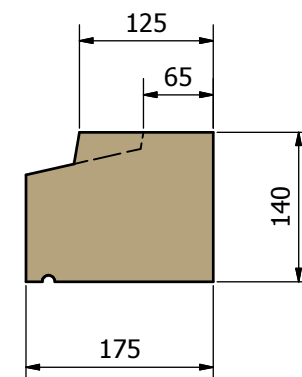
'SR' TYPE SEMI-DRY PROFILE ( 1 : 5 )
