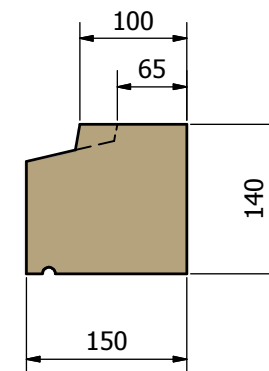
'SC' TYPE SEMI-DRY PROFILE ( 1 : 5 )
