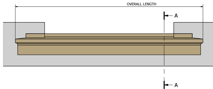
'PWR' TYPE STOOLED CILL (190mm x 140mm) ( 1:5 )
