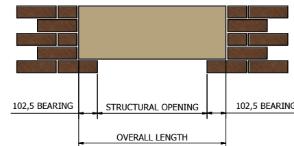
'GH TYPE HEAD' 100mm BED x 290mm HIGH ONE PIECE (OVERALL LENGTH <1547mm)
