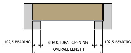
'DHR TYPE HEAD' 120mm BED x 215mm HIGH ONE PIECE (OVERALL LENGTH <1547mm)
