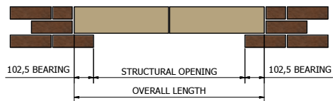
'LH TYPE HEAD' 100mm BED x 140mm HIGH TWO PIECES (OVERALL LENGTH >1547mm)
