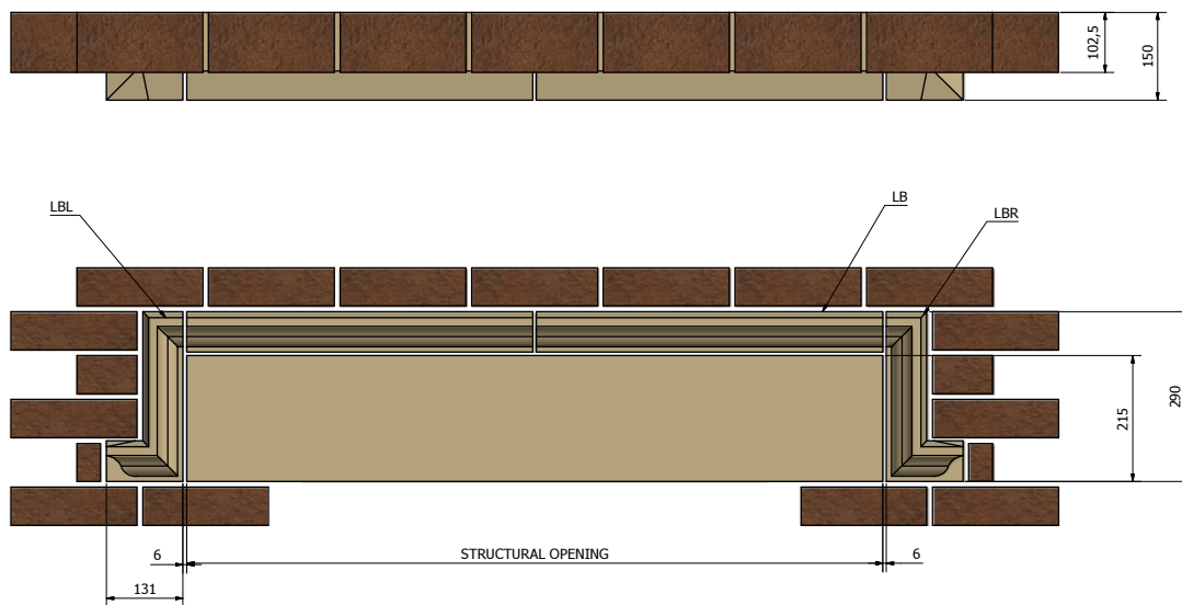
'LB' TYPE LABEL MOULDING OVER 215mm DEEP 'DH' HEAD
