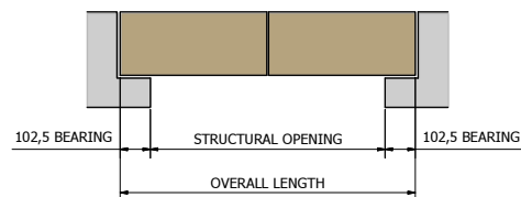
'DHR TYPE HEAD' 120mm BED x 215mm HIGH TWO PIECES (OVERALL LENGTH >1547mm)
