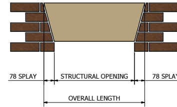
'JH TYPE HEAD' 100mm BED x 290mm HIGH ONE PIECE (OVERALL LENGTH <1000mm)
