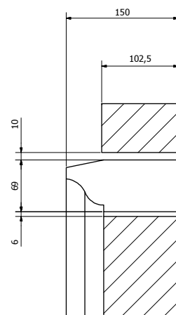
TYPICAL 'LB' SECTION
