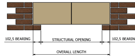
'GH TYPE HEAD' 100mm BED x 290mm HIGH TWO PIECES (OVERALL LENGTH >1547mm)
