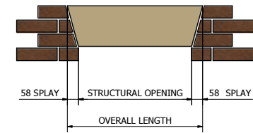
'SH TYPE HEAD' 100mm BED x 215mm HIGH ONE PIECE (OVERALL LENGTH <1000mm)
