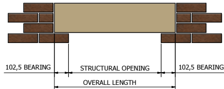
'DH TYPE HEAD' 100mm BED x 215mm HIGH ONE PIECE (OVERALL LENGTH <1547mm)
