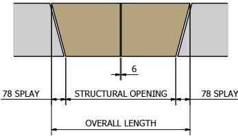
'JHR TYPE HEAD' 120mm BED x 290mm HIGH TWO PIECES (OVERALL LENGTH >1000mm)
