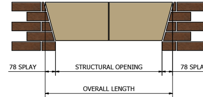
'JH TYPE HEAD' 100mm BED x 290mm HIGH TWO PIECES (OVERALL LENGTH >1000mm)
