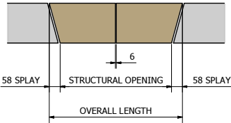
'SHR TYPE HEAD' 120mm BED x 215mm HIGH TWO PIECES (OVERALL LENGTH >1000mm)
