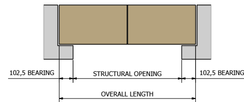
'GHR TYPE HEAD' 120mm BED x 290mm HIGH TWO PIECES (OVERALL LENGTH >1547mm)
