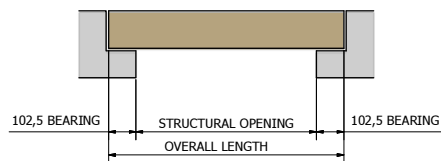
'LHR TYPE HEAD' 120mm BED x 140mm HIGH ONE PIECE (OVERALL LENGTH <1547mm)
