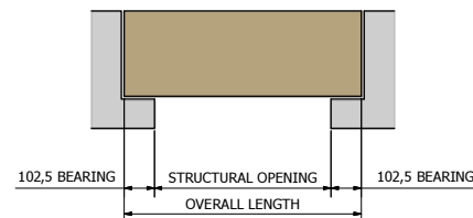
'GHR TYPE HEAD' 120mm BED x 290mm HIGH ONE PIECE (OVERALL LENGTH <1547mm)
