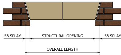
'SH TYPE HEAD' 100mm BED x 215mm HIGH TWO PIECES (OVERALL LENGTH >1000mm)
