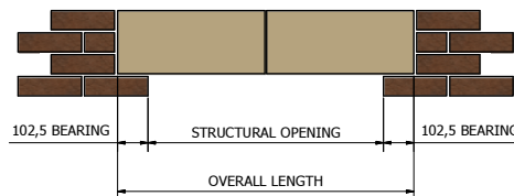
'DH TYPE HEAD' 100mm BED x 215mm HIGH TWO PIECES (OVERALL LENGTH >1547mm)
