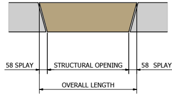
'SHR TYPE HEAD' 120mm BED x 215mm HIGH ONE PIECE (OVERALL LENGTH <1000mm)
