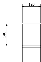
'LHR TYPE HEAD' 120mm BED x 140mm HIGH TWO PIECES (OVERALL LENGTH >1547mm)
