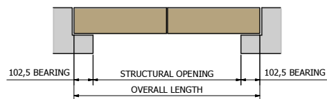
'LHR TYPE HEAD' 120mm BED x 140mm HIGH TWO PIECES (OVERALL LENGTH >1547mm)
