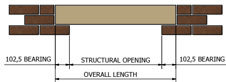
'LH TYPE HEAD' 100mm BED x 140mm HIGH ONE PIECE (OVERALL LENGTH <1547mm)
