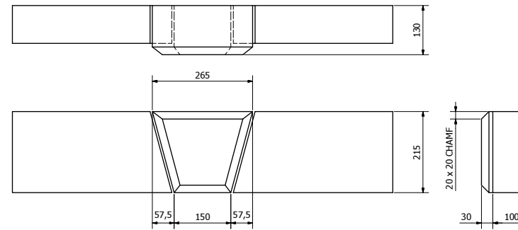
K1C CHAMFERED KEYSTONE IN 215mm HIGH HEAD ( 1 : 5 ) APPROX. 13 KG
