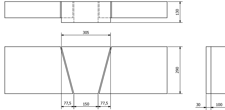
K3 KEYSTONE IN 290mm HIGH HEAD ( 1 : 5 ) APPROX. 20 KG
