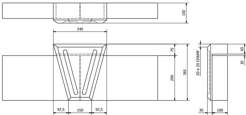
K6F FLUTED KEYSTONE OVER 290mm HIGH HEAD ( 1 : 5 ) APPROX. 12 KG
