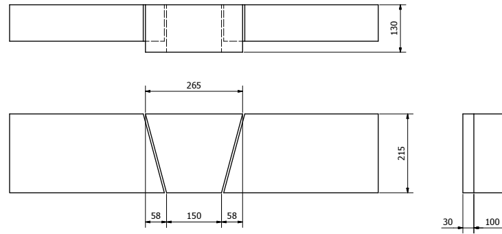
K1 KEYSTONE IN 215mm HIGH HEAD ( 1 : 5 ) APPROX. 14 KG
