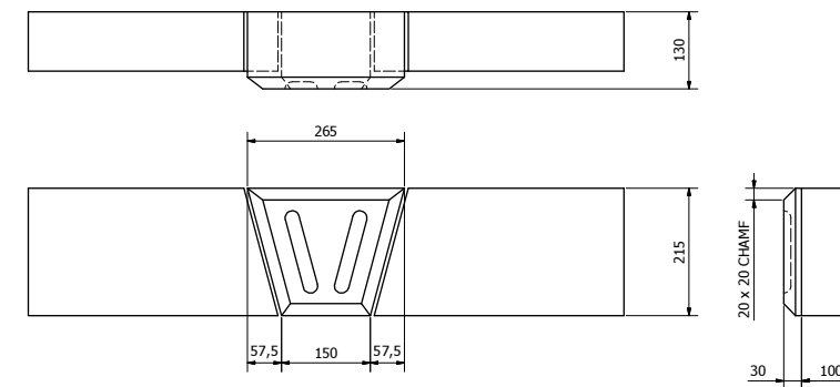
K1F FLUTED KEYSTONE IN 215mm HIGH HEAD ( 1 : 5 ) APPROX. 13 KG
