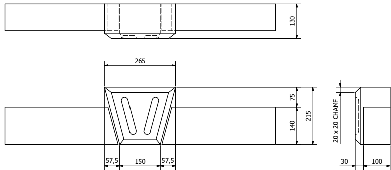
K1F FLUTED KEYSTONE IN 140mm HIGH HEAD ( 1 : 5 ) APPROX. 13 KG
