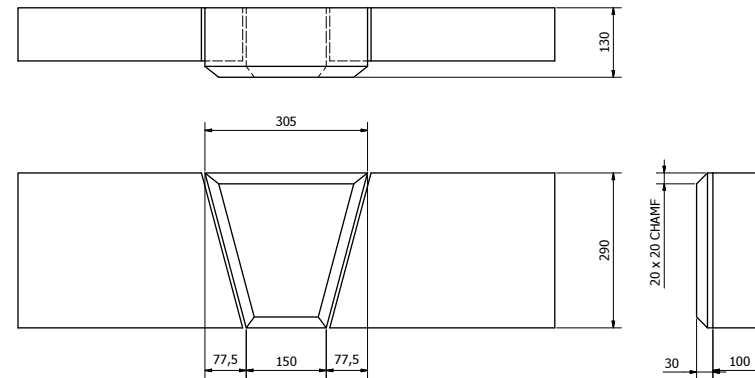
K3C KEYSTONE IN 290mm HIGH HEAD ( 1 : 5 ) APPROX. 20 KG
