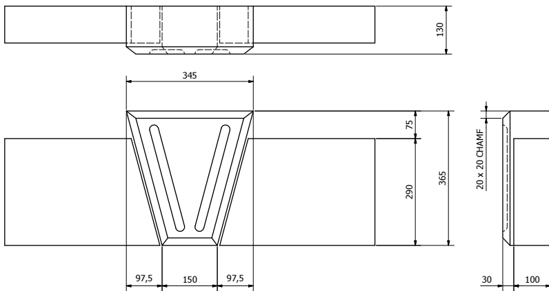
K5F KEYSTONE IN 290mm HIGH HEAD ( 1 : 5 ) APPROX. 27 KG
