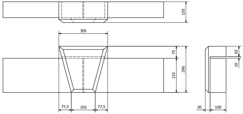
K4C CHAMFERED KEYSTONE OVER 215mm HIGH HEAD ( 1 : 5 ) APPROX. 9 KG
