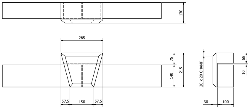
K2C CHAMFERED KEYSTONE OVER 140mm HIGH HEAD ( 1 : 5 ) APPROX. 7 KG
