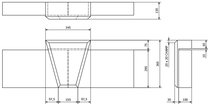
K6C CHAMFERED KEYSTONE OVER 290mm HIGH HEAD ( 1 : 5 ) APPROX. 12 KG
