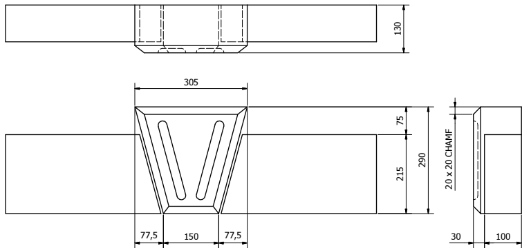
K3F KEYSTONE IN 215mm HIGH HEAD ( 1 : 5 ) APPROX. 20 KG
