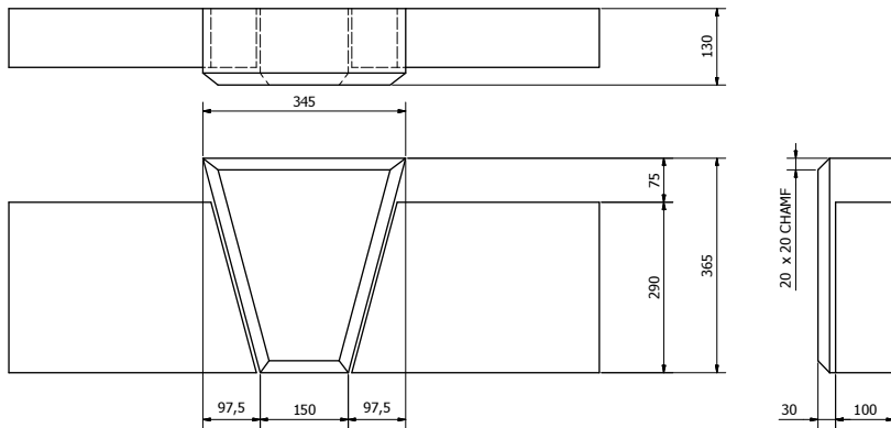
K5C KEYSTONE IN 290mm HIGH HEAD ( 1 : 5 ) APPROX. 27 KG
