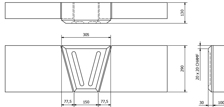
K3F KEYSTONE IN 290mm HIGH HEAD ( 1 : 5 ) APPROX. 20 KG
