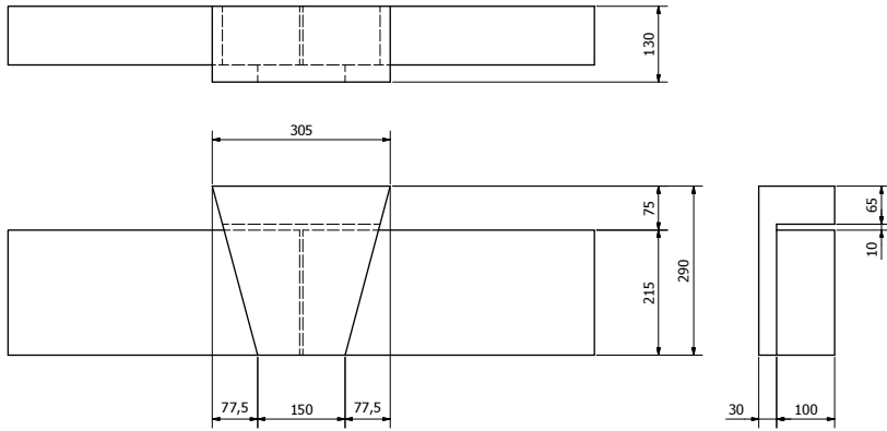
K4 KEYSTONE OVER 215mm HIGH HEAD ( 1 : 5 ) APPROX. 9 KG
