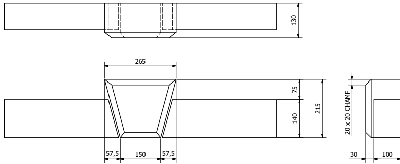
K1C CHAMFERED KEYSTONE IN 140mm HIGH HEAD ( 1 : 5 ) APPROX. 13 KG
