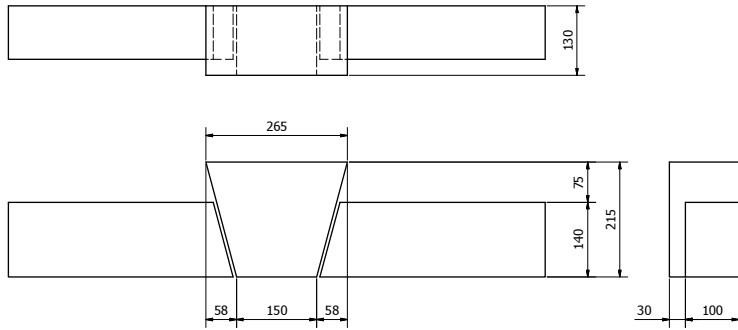
K1 KEYSTONE IN 140mm HIGH HEAD ( 1 : 5 ) APPROX. 14 KG
