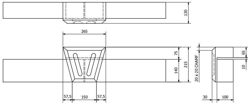
K2F FLUTED KEYSTONE OVER 140mm HIGH HEAD ( 1 : 5 ) APPROX. 7 KG
