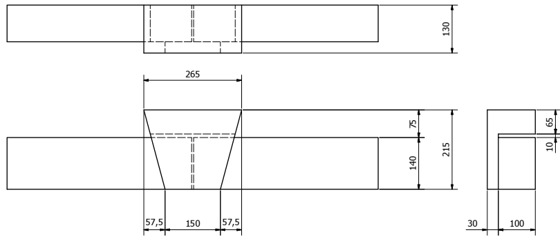
K2 KEYSTONE OVER 140mm HIGH HEAD ( 1 : 5 ) APPROX. 7 KG
