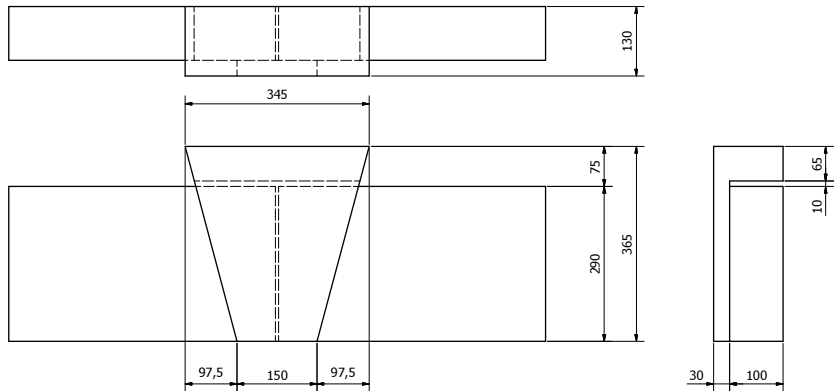
K6 KEYSTONE OVER 290mm HIGH HEAD ( 1 : 5 ) APPROX. 12 KG
