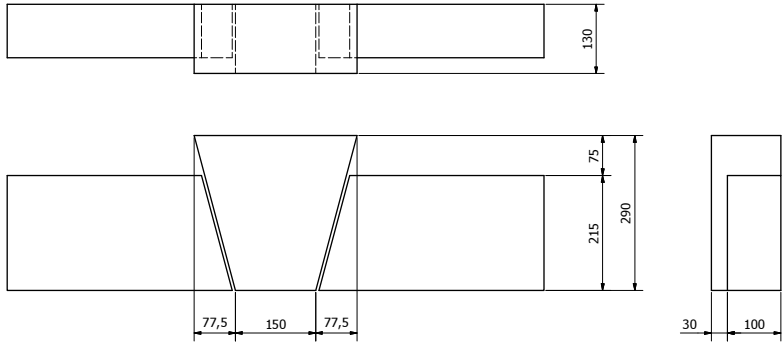
K3 KEYSTONE IN 215mm HIGH HEAD ( 1 : 5 ) APPROX. 20 KG
