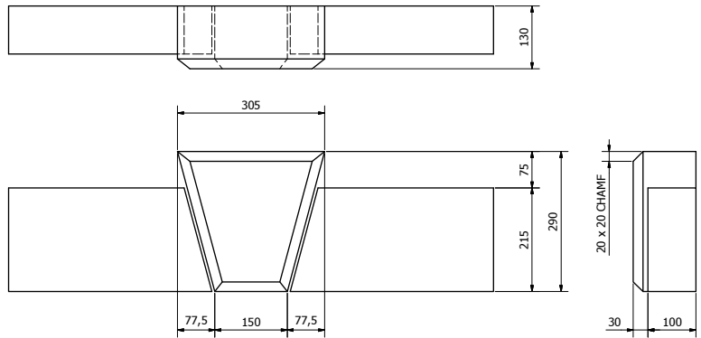
K3C KEYSTONE IN 215mm HIGH HEAD ( 1 : 5 ) APPROX. 20 KG
