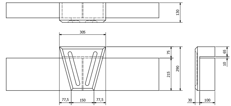
K4F KEYSTONE OVER 215mm HIGH HEAD ( 1 : 5 ) APPROX. 9 KG
