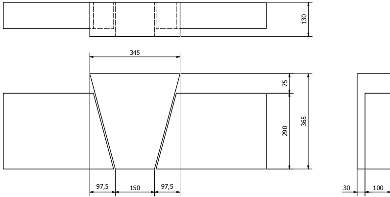
K5 KEYSTONE IN 290mm HIGH HEAD ( 1 : 5 ) APPROX. 27 KG
