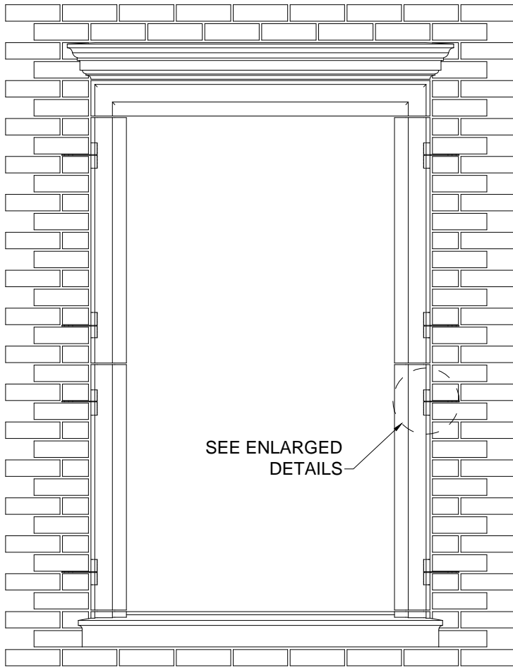
TYPICAL ELEVATION
