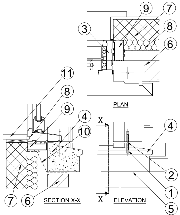
ENLARGED DETAILS
