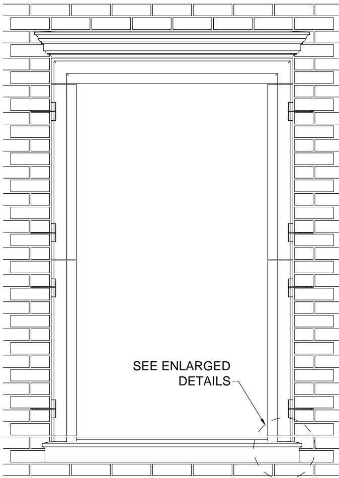
TYPICAL ELEVATION
